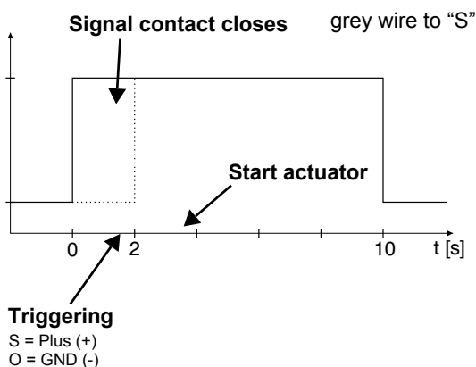
Figure 1: Signal contact diagram – driving direction OPEN
