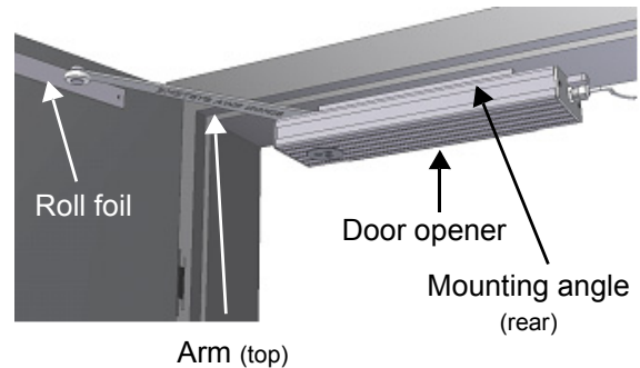
Figure 14: Rear view – DIN “left” door
